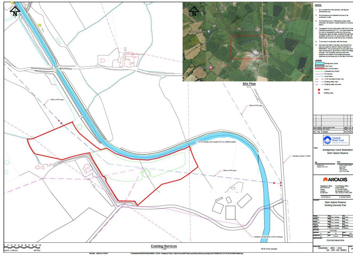
Fig. 6: Detailed Existing Service Plan of the Site
