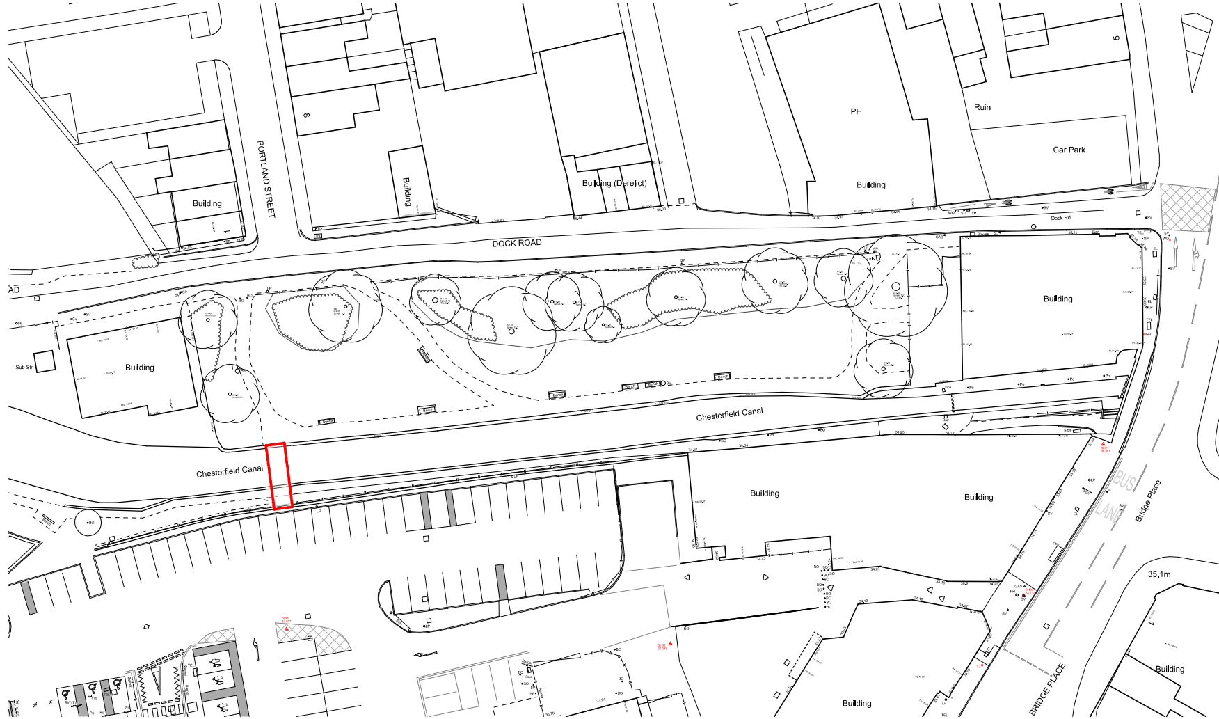
Pedestrian Bridge Location 1:500
