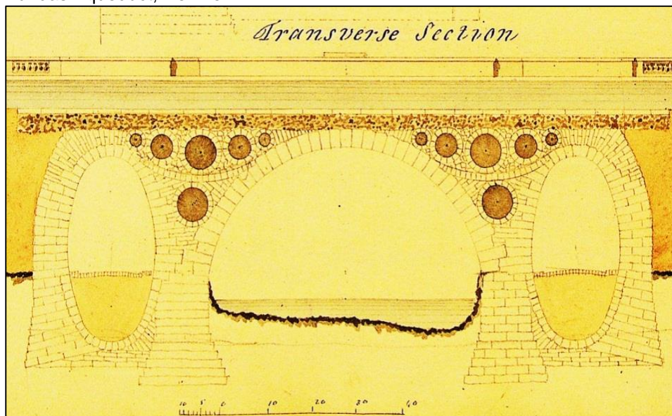
Dundas Aqueduct, Rennie
