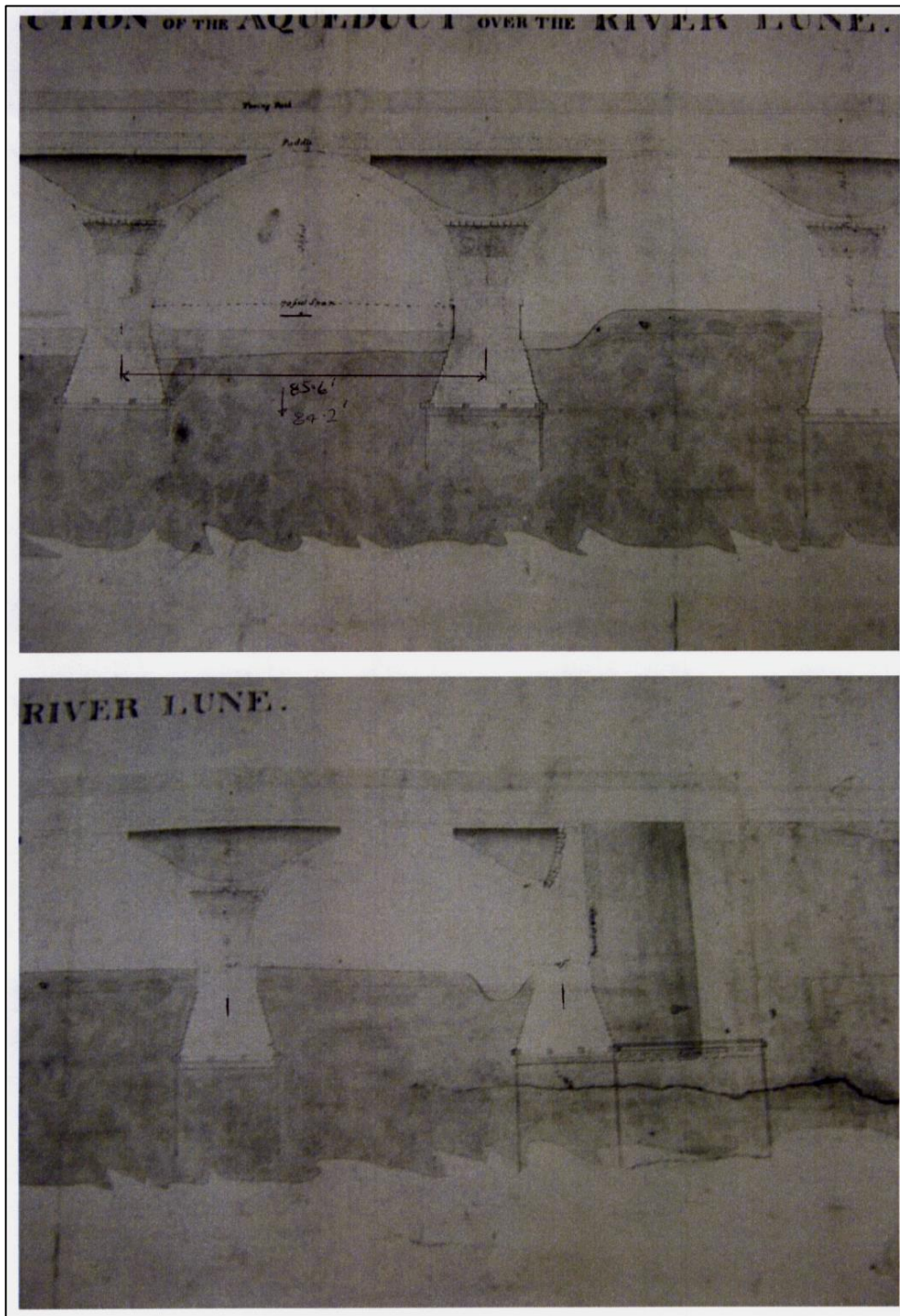
Lune Aqueduct, Rennie 1795
